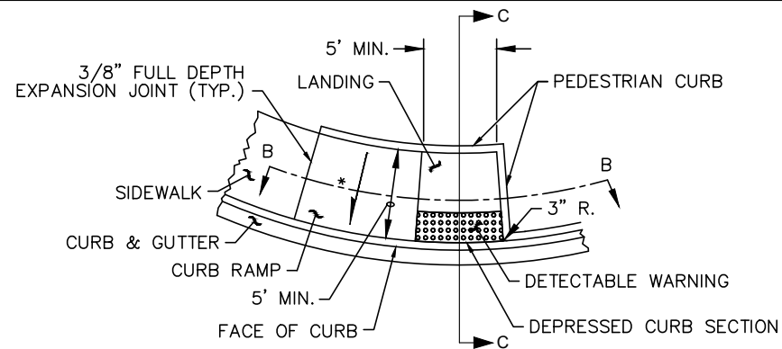
CURB RAMP TYPE PARALLEL B
