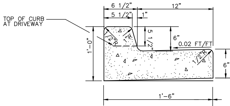
CEMENT CONCRETE TRAFFIC CURB AND GUTTER
