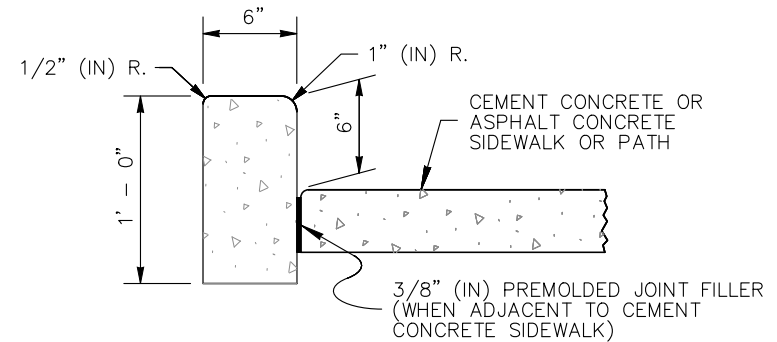
CEMENT CONCRETE PEDESTRIAN CURB
