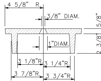
SECTION COVER
