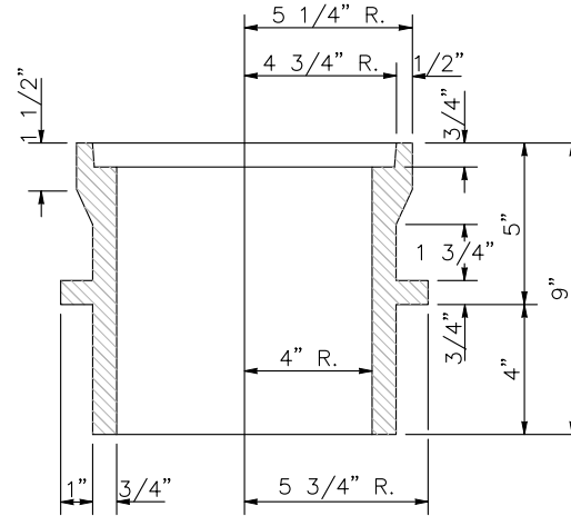
SECTION CASE
