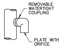
ELBOW DETAIL
