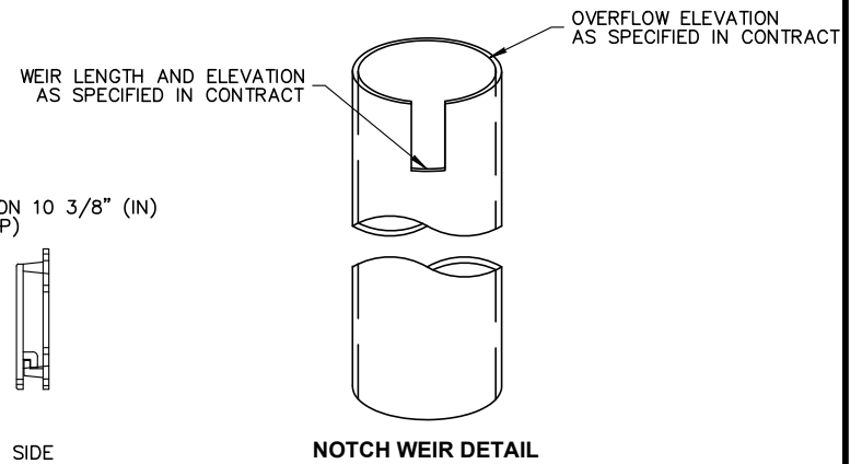
NOTCH WEIR DETAIL
