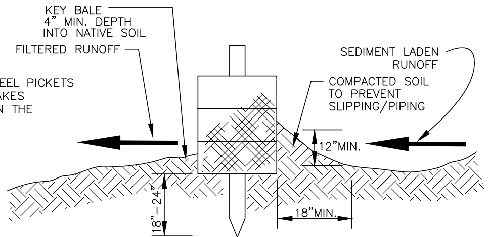
CROSS-SECTION OF STRAW BALE
