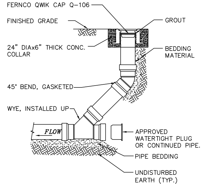
CLEANOUT WITH CONCRETE COLLAR
