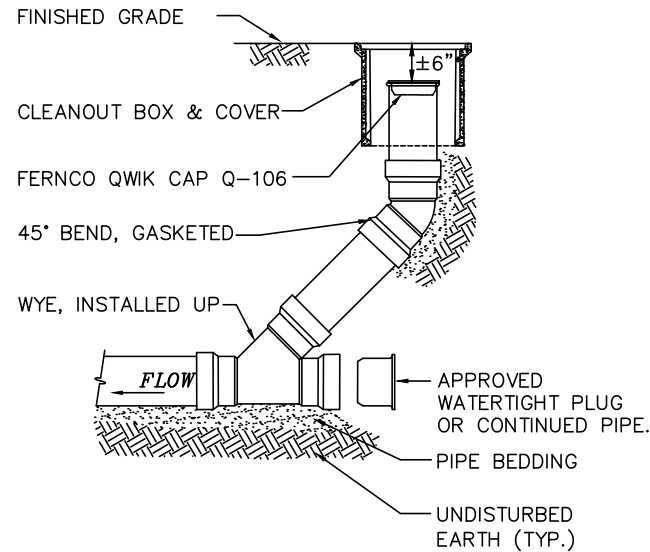
CLEANOUT IN BOX
