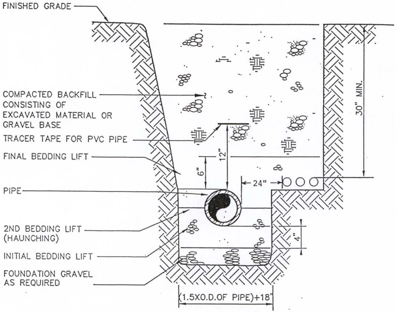
UTILITY TRENCH SECTION
